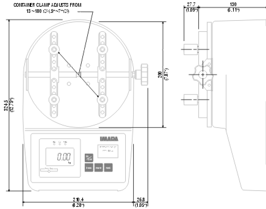
DTX DIMENSIONS
