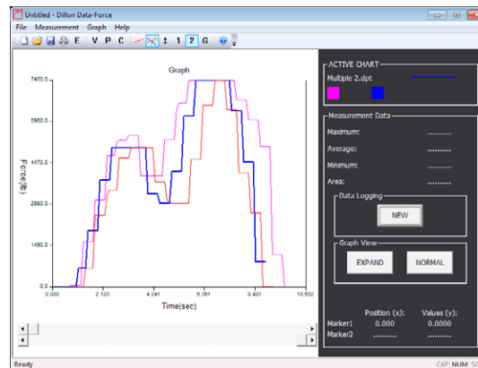
Multi-trace display
